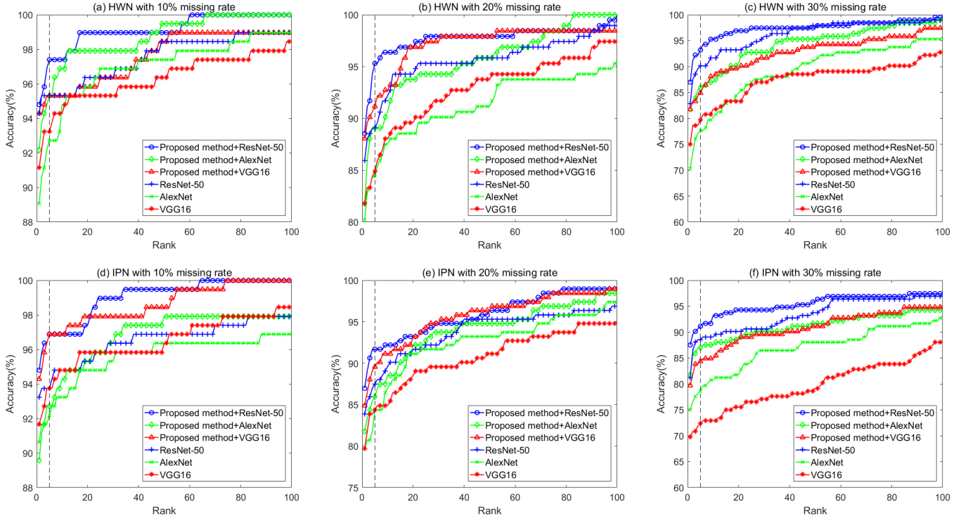
Fig. 7. CMC curves on the XJTU-UP databases: (a-c) are the CMC curves on the HWN dataset with missing rates of 10%, 20%, and 30%, respectively. (d-f) are the CMC curves on the IPN dataset with missing rates of 10%, 20%, and 30%, respectively. (The dotted line represents rank=5.)
