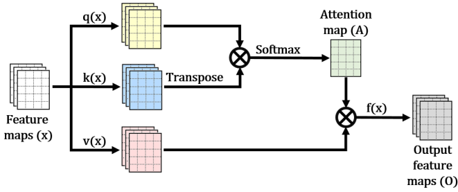
Fig. 3. The framework of self-attention model, where \otimes denotes matrix multiplication.
